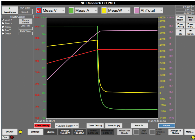
FIGURE 3 Chart Recorder
