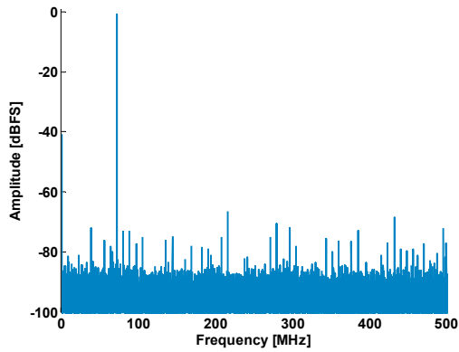
Figure 3: ADQ8-8C 50 Ω frequency domain plot.
