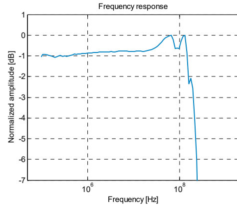
Figure 2: ADQ8-8C 1 MΩ frequency response.
