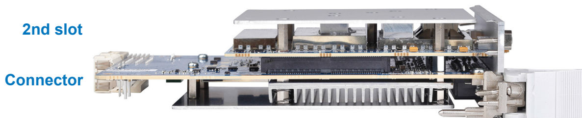
Figure 7: ADQ7WB-PXIE extends to the left of the connector. Bottom view with the handle to the right.
