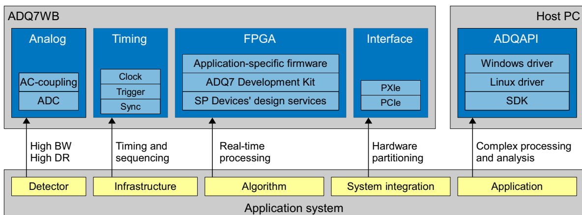
Figure 4: Integrating the ADQ7WB into the system.
