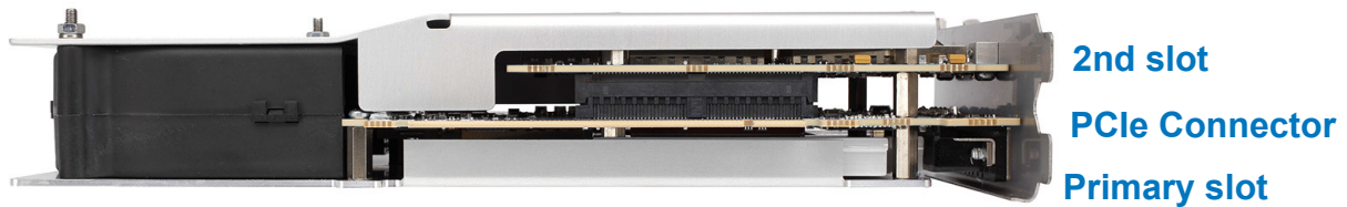
Figure 10: ADQ7WB–PCIE extends to the left of the connector.
