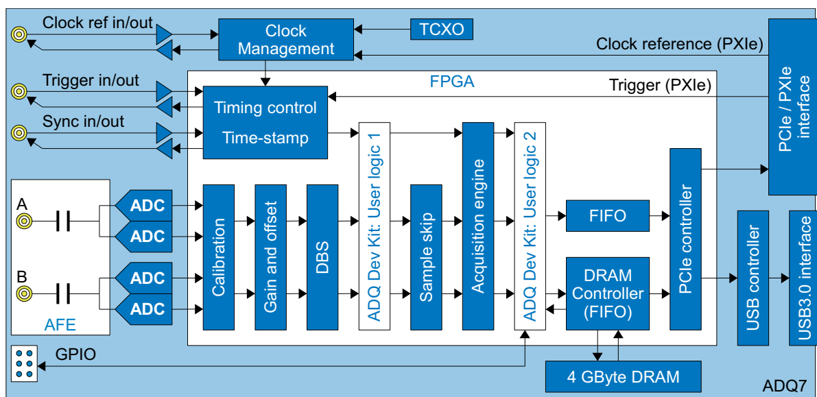
Figure 5: Block diagram for ADQ7WB–FWDAQ (standard firmware).
