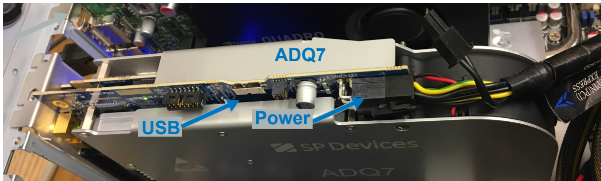
Figure 9: ADQ7WB installed in a PC. Note the power supply cable.
